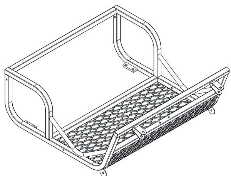
A x1
